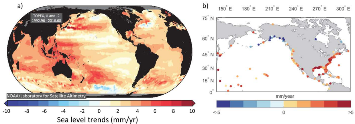
Figure 4. a) Sea level change rates from 1992–2016 from TOPEX/Poseidon, Jason-1 and Jason-2 ( www.star.nesdis.noaa.gov/sod/lssa/SeaLevelRise ) and b) relative sea level trends based upon full record ( >30 -year period of record in all cases) measured and published for NOAA tide gauges through 2015 ( tidesandcurrents.noaa.gov/sltrends ).
